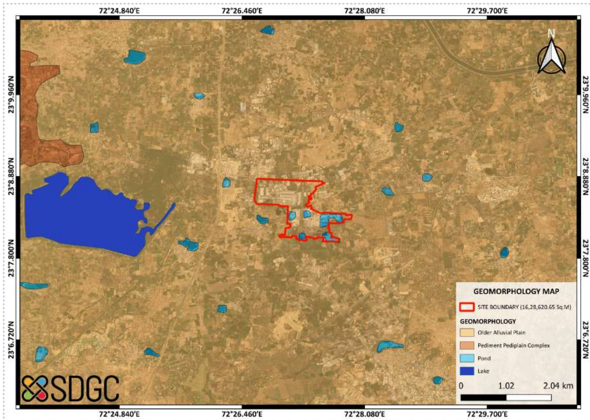
Figure 9.1: Geomorphology Map
