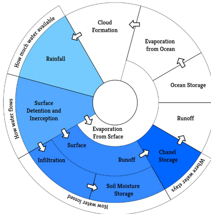
Figure 5.1: Ancient Hydrological Cycle from 800 to 500 B.C.
