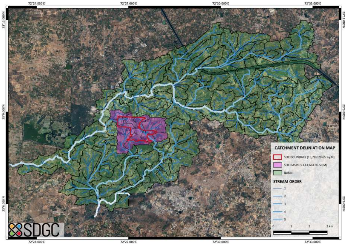
Figure 8.3: Catchment Delineation Map
