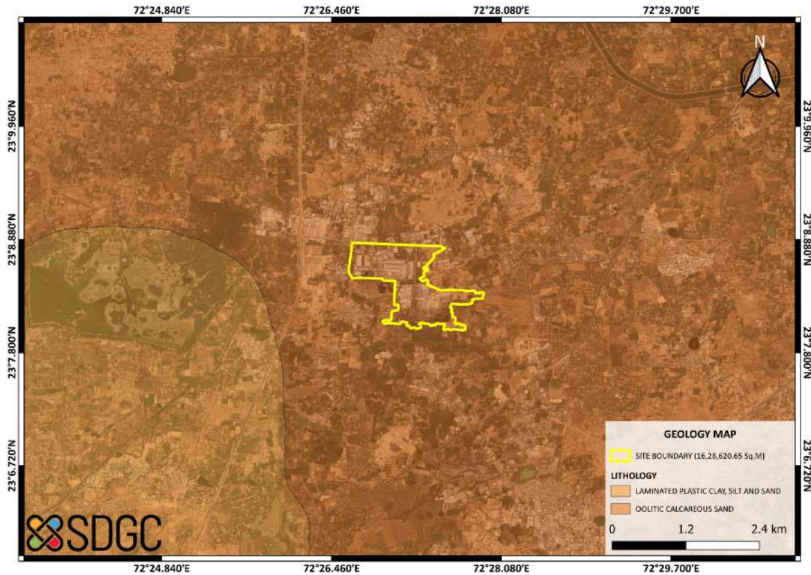
Figure 9.2: Regional Level Geology Map
